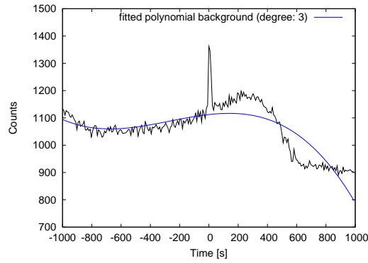
Figure 1: Lightcurve of the Fermi-burst 091030613 measured by the 3rd GBM detector. The burst is at 0 s but the variation of the background is comparable with its height, and cannot be modelled by a simple polynomial function of time of degree 2 or 3.
