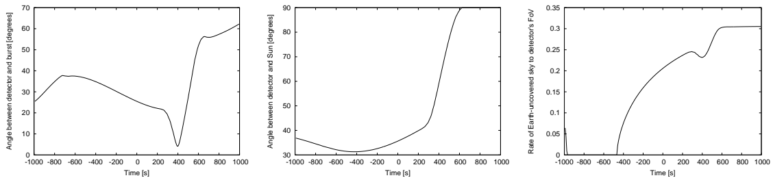
Figure 2: From left to right: The celestial distance of the 3rd GBM detector and the position of Fermi-burst 091030613; the same with the Sun; and the rate of the Earth-uncovered sky to the 3rd GBM detector's field of view, both in the function of time. It is worth comparing these figures with Fig. 1.
