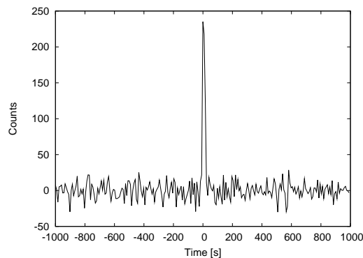
Figure 3: After background fitting: the lightcurve of Fermi-burst 091030613 measured by the 3rd GBM detector. Comparing Fig. 1 to Fig. 3, we can state that our background filtering was successful, since the resulting lightcurve is perfectly background-free.
