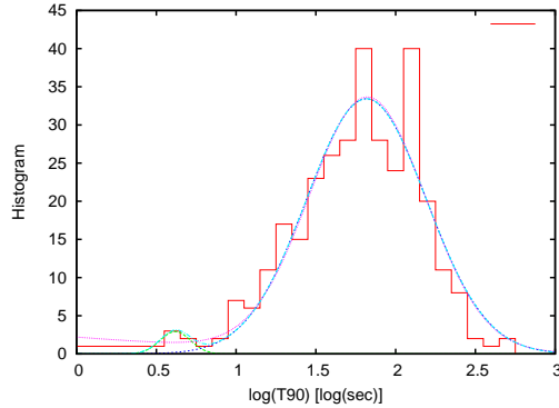
Figure 4: The distribution of the \log T_{90} statistical parameter for 332 bursts according to our method. The coloured curves show the fitted Gaussian functions: green and blue for the short peak and the long peak, light blue and purple for together.
