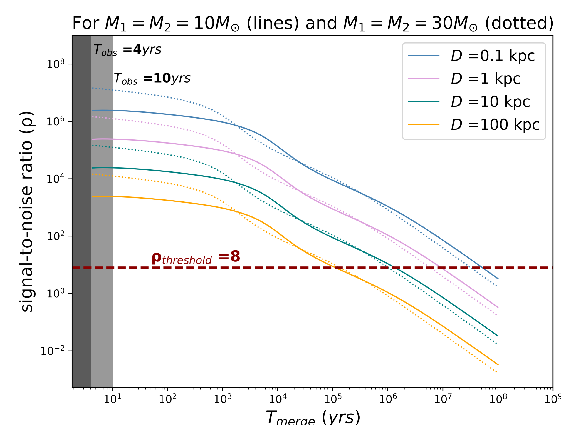
Figure 2: The plot shows the signal to noise ratio ( \rho ) for black holes binaries of m_1 = m_2 = 10M_\odot (lines) and m_1 = m_2 = 30M_\odot (dotted) as a function of their merger times T_{merge} (yrs) with LISA for different distances from 0.1kpc to as far as 100kpc. The horizontal (dashed) red line represents here the detection threshold of SNR \rho_{thr} = 8 whereas the vertically shaded black and grey regions represent LISA observing times T_{obs} = 4 years.
