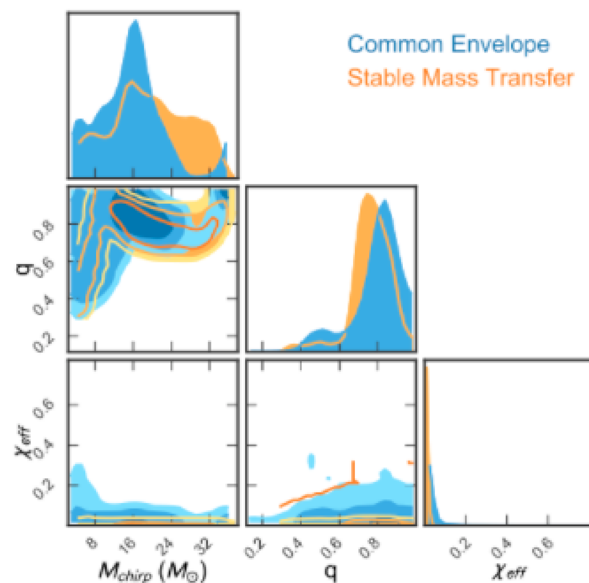
Figure 1: The distribution of observable properties of BBH chirp mass, \chi_{eff} and mass ratio q , that would merge within the next 20 years.
